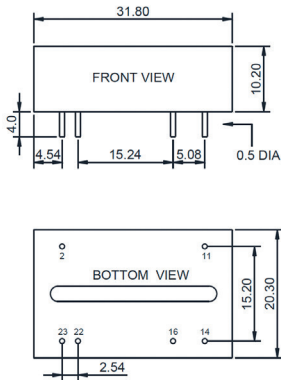
PIN Connection
