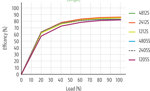
Efficiency vs load (Single)
