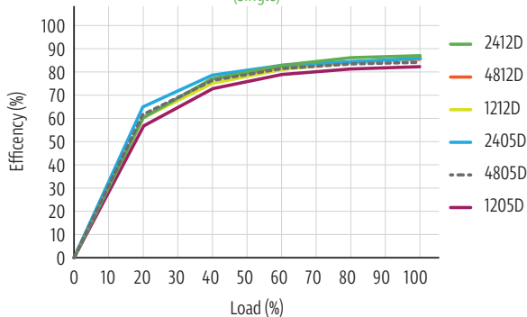
Efficiency vs load (Single)
