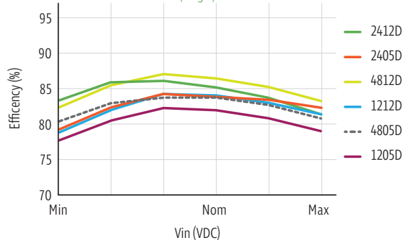
Efficiency vs vin (Single)
