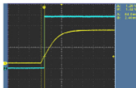
CH1: Vin/off CH2: Vo Delay time: 64mS
