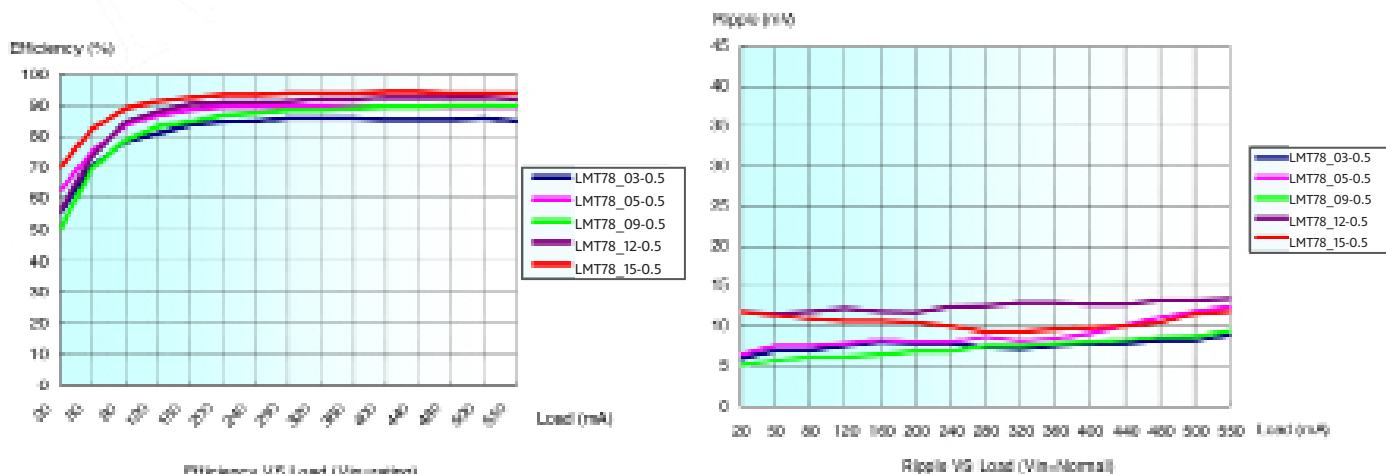
Efficiency VS Output Load (Vin=Norm)
