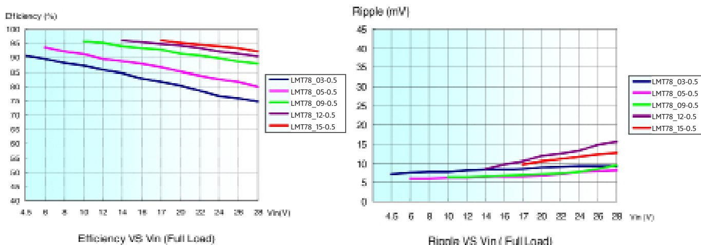
Efficiency VS Input Voltage (Full Load)
